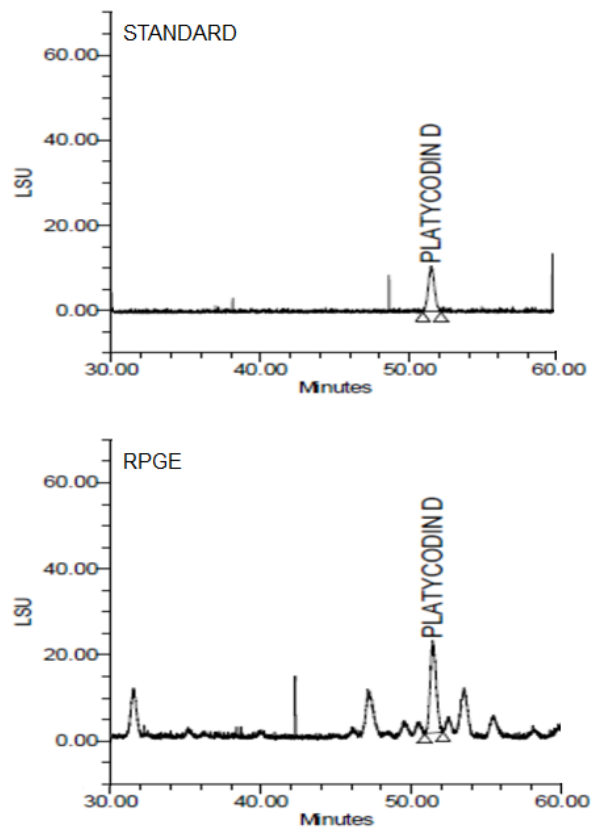
Fig. 1. Chromatograms of active ingredients in Red Platycodon grandiflorum Extract (RPGE)
