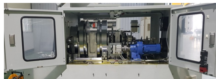
Fig. 5. Brake dynamometer mechanical part
