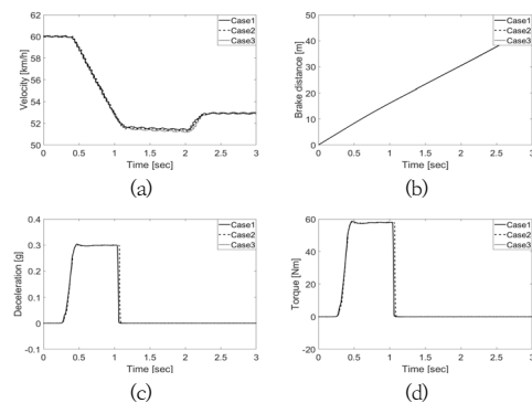
Fig. 13. Brake dynamometer test results for LKAS (a) Velocity (b) Brake distance (c) Deceleration (d) Torque
