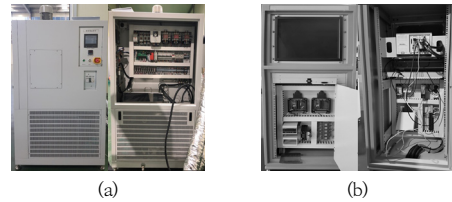
Fig. 8. Brake dynamometer part (a) Environment part (b) Controller
