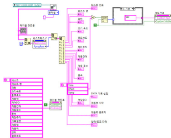
Fig. 9. Test code edit block diagram
