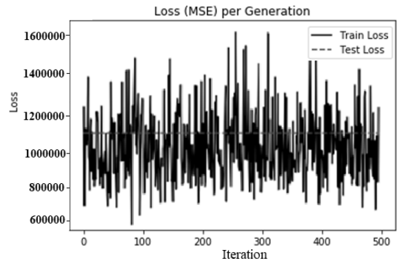
Fig. 7. Experimental Results with Gradient Descent Optimizer
