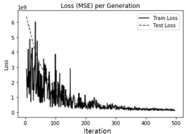
Fig. 5. Experimental Results in a Batch with the Size of 20
