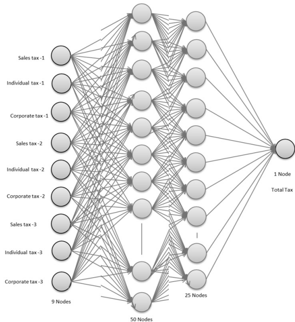
Fig. 1. Topology of Artificial Neural Network Model in the Experiment
