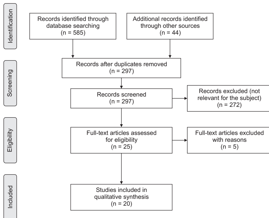
Figure 1. PRISMA diagram.
