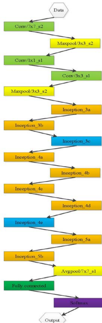
Fig. 3. Inception-v2 structure
