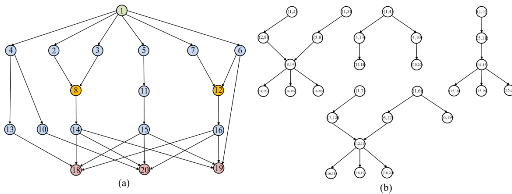
Fig. 11(a) Multicast session for G with 18 nodes. (b) Directed Labeled Line Graph for G with 18 nodes.
