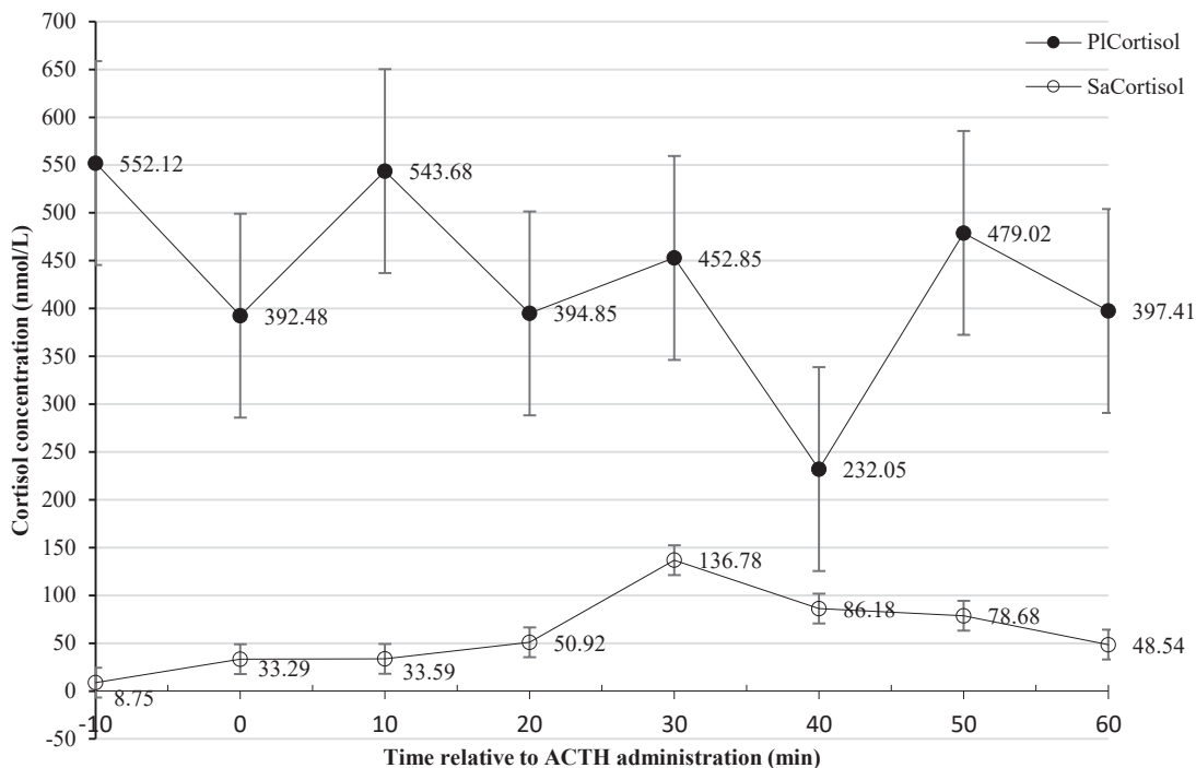
Figure 2. Cortisol concentrations of cows subjected to a hormonal challenge using a standardised dose (1 µg/kg) of adrenocorticotrophic hormone at time 0. Line graphs represent plasma cortisol (● PICortisol) and salivary cortisol (⊕ SaCortisol) concentrations. Line graphs represent cortisol concentrations which either increased or decreased as depicted by the down-up or up-down lines respectively and the error bars represent the standard error of means. Insignificant differences were observed for plasma concentrations in contrast to the saliva concentrations which were variable ( p < 0.001 ).
