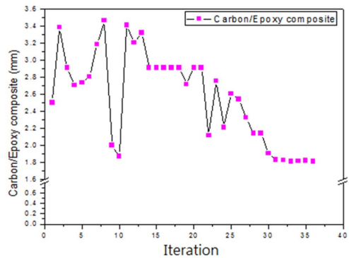
(c) Thickness result of T700 carbon/epoxy composite
