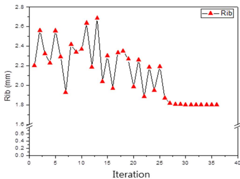
(a) Thickness result of rib
