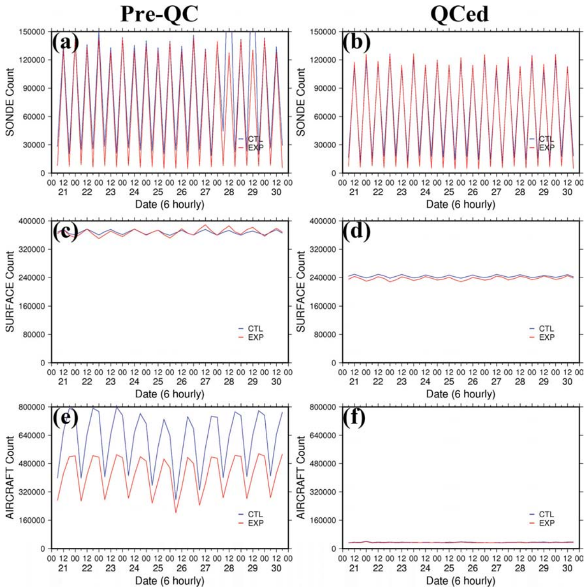
Fig. 4. Time series of Pre-QC (left column) and QCed (right column) observation number of (a, b) SONDE, (c, d) SURFACE, and (e, f) AIRCRAFT for CTL (blue solid line) and EXP (red solid line) during 9 days (from 2018.03.21 0600 UTC to 2018.03.30 1800 UTC). Counted value represents the sum of meteorological variables.
