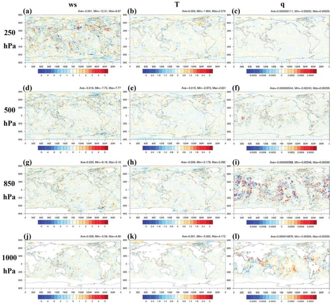
Fig. 9. Horizontal error reduction difference between CTL and EXP against IFS for (a, d, g, j) wind speed, (b, e, h, k) T, and (c, f, i, l) q for (first row) 250 hPa, (second row) 500 hPa, (third row) 850 hPa, and (fourth row) 1000 hPa at 2018.03.29 0000 UTC. Red color means that EXP shows better forecast performance than CTL.
