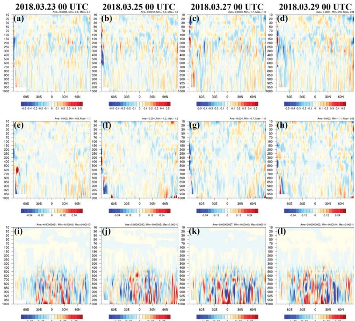
Fig. 10. Vertical error reduction difference between CTL and EXP against IFS for (a, b, c, d) wind speed, (e, f, g, h) T, and (i, j, k, l) q at (first column) 2018.03.23 0000 UTC, (second column) 2018.03.25 0000 UTC, (third column) 2018.03.27 0000 UTC, and (fourth column) at 2018.03.29 0000 UTC. Red color means that EXP shows better forecast performance than CTL.
