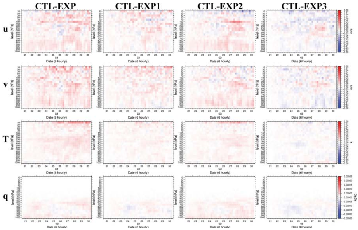
Fig. 8. Time series of vertical RMSD difference between CTL and EXPs against IFS for u, v, T, and q. Red color means that EXPs shows better forecast performance than CTL.
