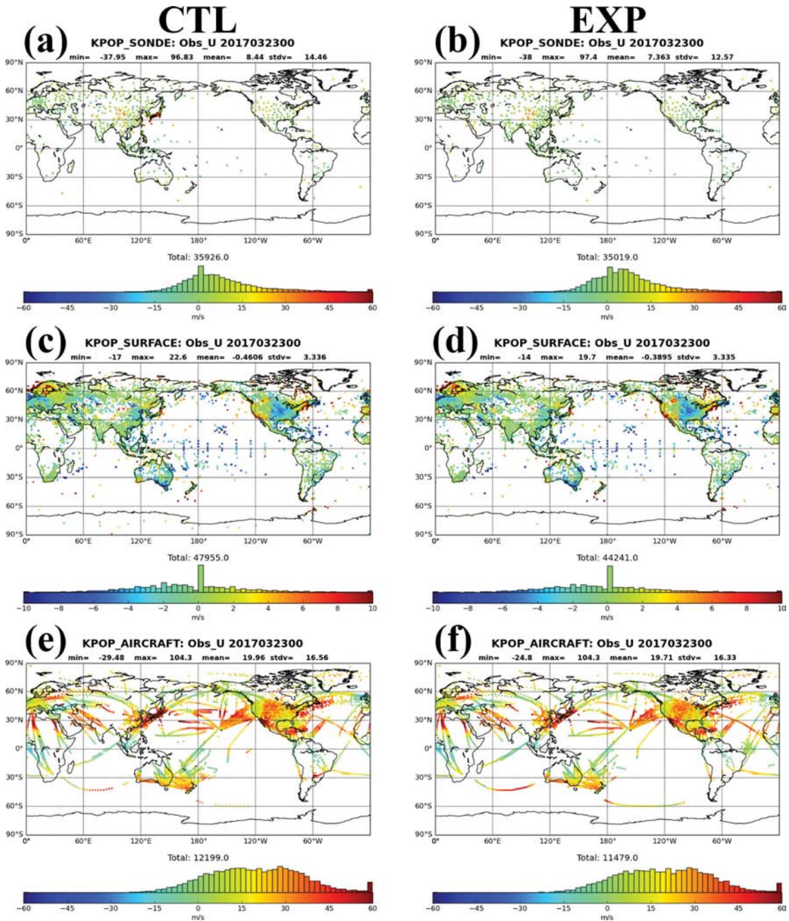
Fig. 2. The same as the Fig. 1, but for the u wind after KPOP processing.
