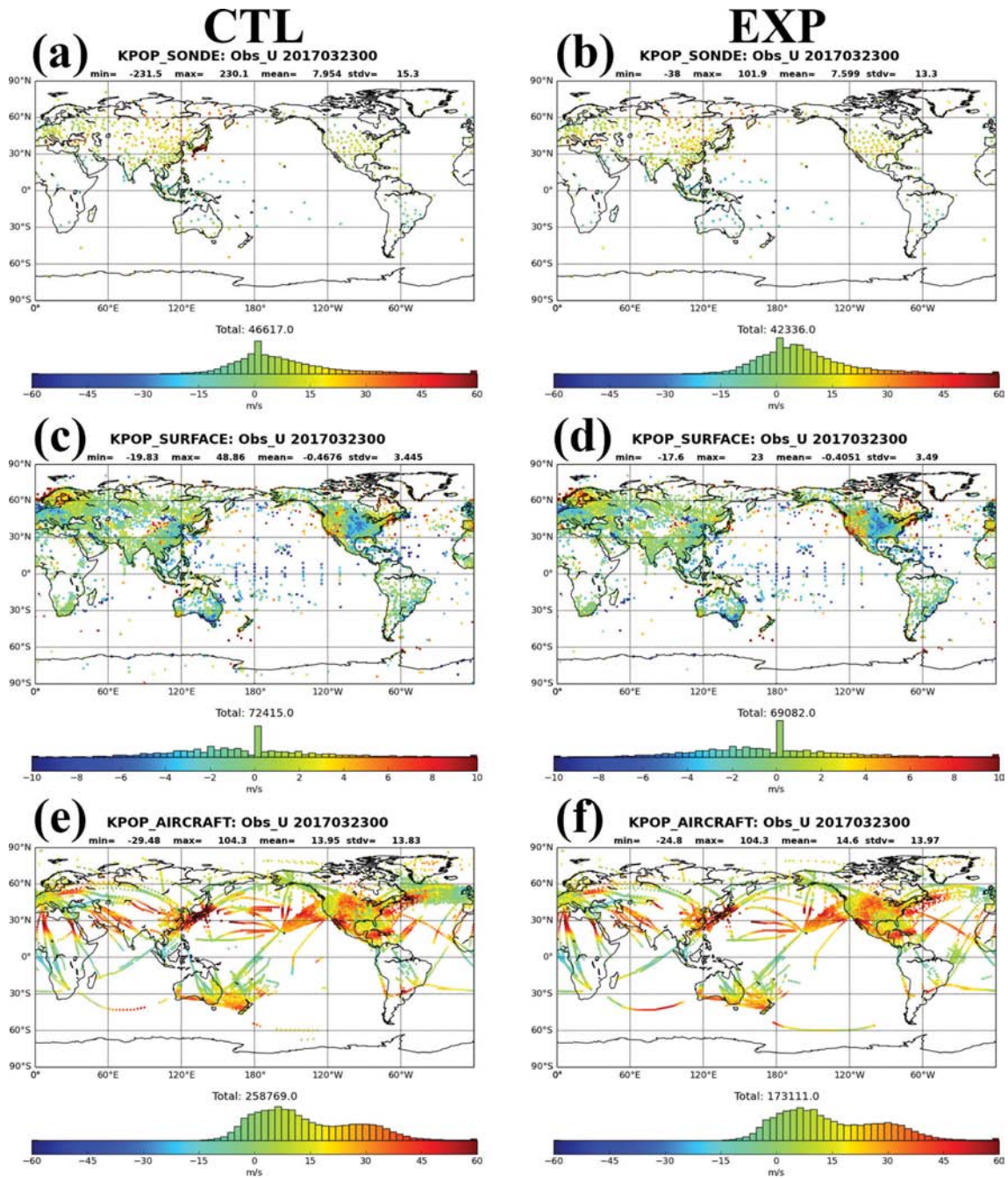
Fig. 1. Global distribution of u wind before KPOP processing for (left column) CTL and (right column) EXP, for (a, b) SONDE, (c, d) SURFACE, and (e, f) AIRCRAFT at 2017.03.23 0000 UTC. The histogram shows the cumulative number of observations based on wind speed.
