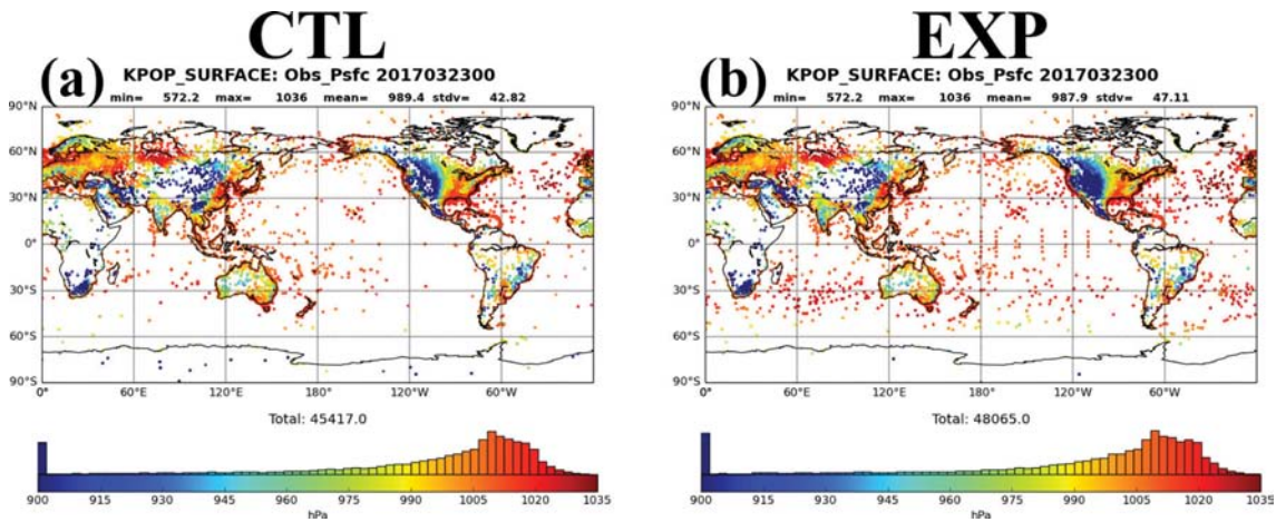
Fig. 3. Global distribution of Ps after KPOP processing for (left) CTL and (right) EXP, for SURFACE at 2017.03.23 0000 UTC. The histogram shows the cumulative number of observations based on surface pressure.
