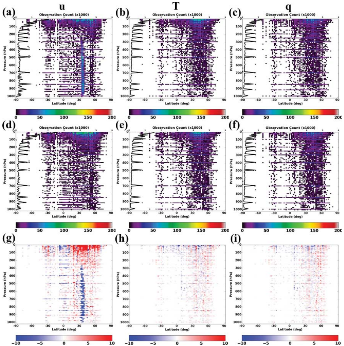
Fig. 5. Vertical distribution (point) of SONDE for (a, d) u, (b, e) T, and (c, f) q on (upper) CTL, and (middle) EXP at 2018.03.23 0000 UTC and sum of points at each 10 hPa (black line). Lower panel shows the difference of observation count between CTL and EXP for (g) u, (h) T, and (i) q (red color means that EXP have more observations than CTL).
