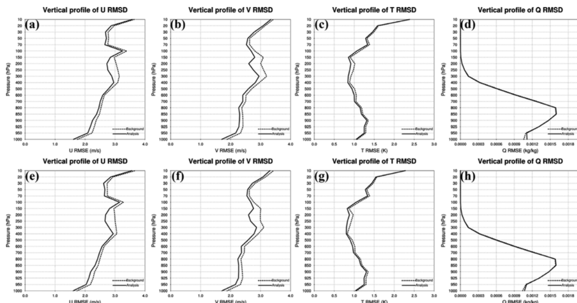
Fig. 6. Vertical profile of global mean RMSD against IFS for (a, e) u, (b, f) v, (c, g) T, and (d, h) q on (upper) CTL and (lower) EXP at 2018.03.29 0000 UTC.
