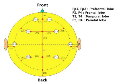
Fig. 2. International 10-20 System
