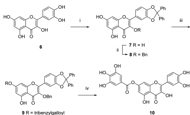
Scheme 2. Synthesis of quercetin-7-gallate.
