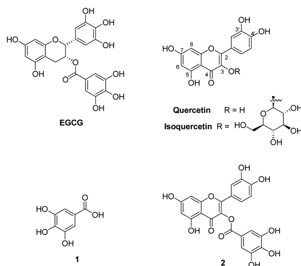
Figure 1. Chemical structures of EGCG, quercetin, isoquercetin, gallic acid (1) and quercetin-3-gallate (2).
