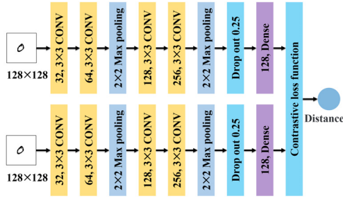
(Figure 4) Siamese model for writer verification
