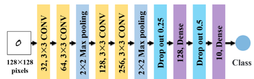
(Figure 3) CNN model for handwriting recognition
