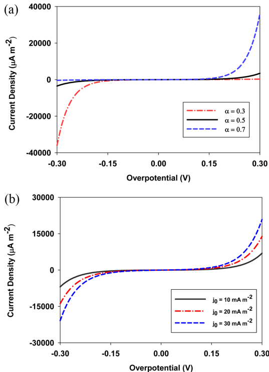
Fig. 2. (a) Overpotential – Current density graph with symmetry factor change, (b) Overpotential – Current density graph with change of equilibrium exchange current density.
