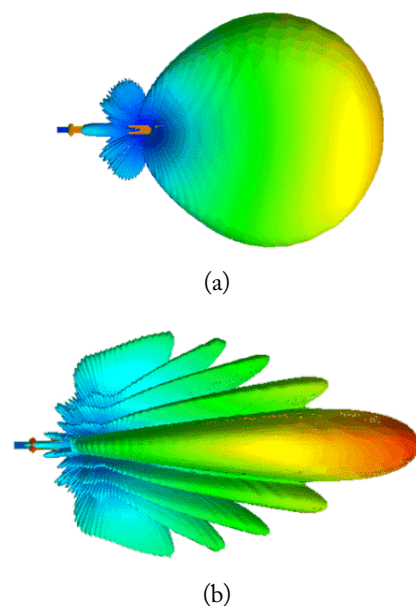
Fig. 7. Comparison of the 3D patterns of the antenna. (a) Vertical and horizontal HPBWs of 50^\circ and 40^\circ (max. cost antenna) and (b) vertical and horizontal HPBWs of 10^\circ and 60^\circ (min. cost antenna).
