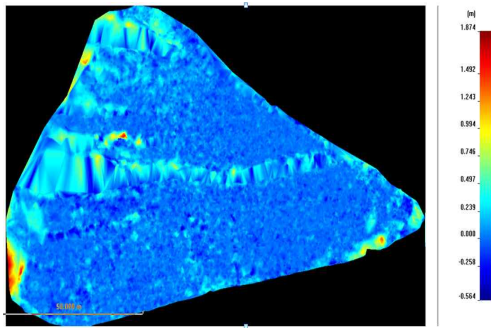
Fig. 10. Amount of Change by Mesh Overlay - Slope 1
