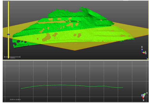
Fig. 7. Section Created using Pointcloud
