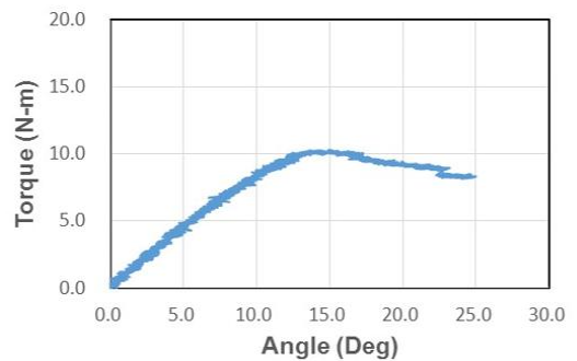
Fig 9. Torsional response for M30-3
