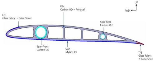
Fig 1. Typical wing cross section
