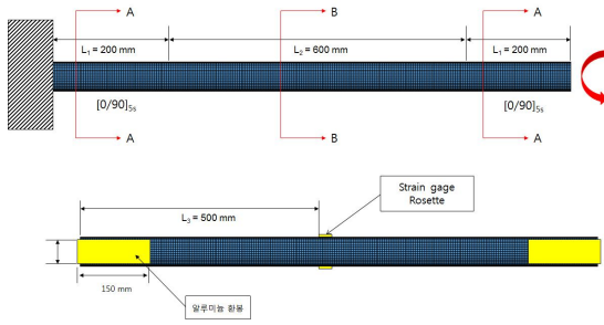
Fig 5. Dimension of test specimen
