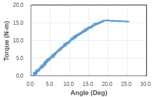
Fig 10. Torsional response for M30-4
