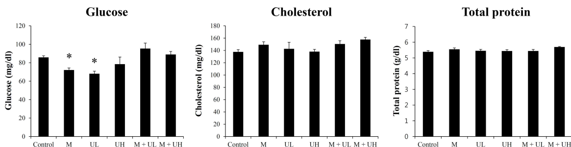
Fig. 1. Change of organic serum components (glucose, cholesterol, and total protein) in rainbow trout ( Oncorhynchus mykiss ) after treatment of ultrasonic and microbubble. Asterisk (*) means that there is statistical significance (P<0.05) to the control. M, microbubble treatment for 30 sec; UL, low intensity ultrasonic treatment at 40kHz, 280W for 30 sec; UH, high intensity ultrasonic treatment at 40kHz, 400W for 30 sec; M + UL, microbubble and low intensity ultrasonic treatment at 40kHz, 280W for 30 sec; M + UH, microbubble and high intensity ultrasonic treatment at 40kHz, 400W for 30 sec.
