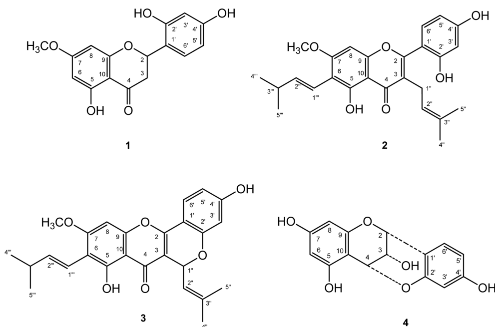
Fig. 1. Chemical structure of flavonoids isolated from A. heterophyllum heartwoods, artocarpanone (1), artocarpin (2), cycloartocarpin (3), and cyanomaclurin (4).
