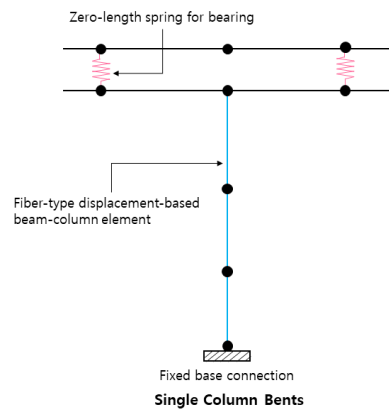
Fig. 6 Modeling of the pier and bearings
