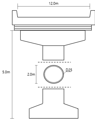
Fig. 4 Pier of the representative bridge
