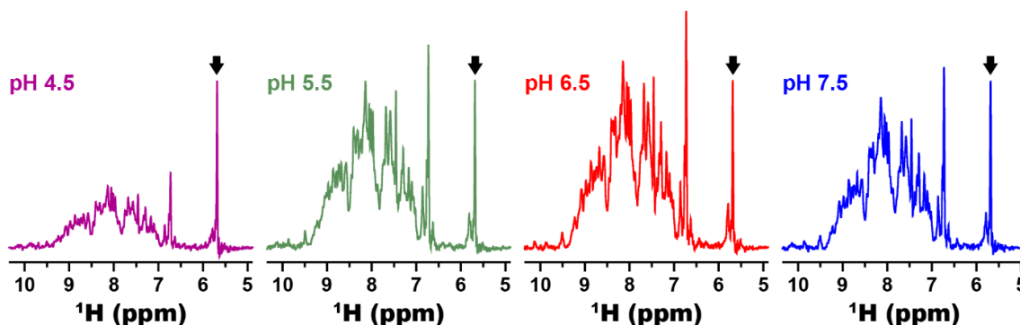
Figure 1. 1D ^1\text{H} - ^{15}\text{N} HSQC spectra of the refolded ^{15}\text{N} -Blvrb protein at different conditions. The 1D ^1\text{H} - ^{15}\text{N} HSQC spectra were recorded with 3017 number of scans. The peak of natural abundant 15 mM urea is indicated with an arrow. The optimal pH values of the buffer seem to be 5.5~6.5 for the optimal refolding of ^{15}\text{N} -Blvrb protein. Each refolding buffer contained each 50 mM buffer component, 0.4 M arginine, and 1 mM DTT.
