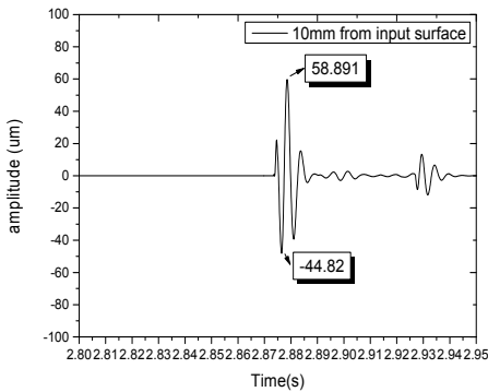
Fig. 12. Amplitude of 10mm point from input surface
