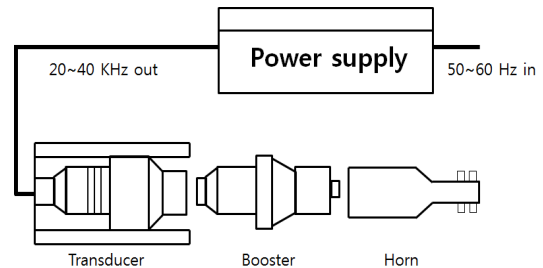
Fig. 1. Ultrasonic welding process setup
