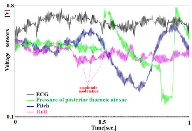
Fig. 11. Correlation between ECG, posterior thoracic air sac pressure, and angular velocity (pitch, roll) after flight.
