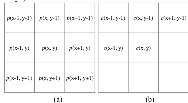
Fig. 4. Pixels which have an effect on the determination of a threshold for c(x, y) ; (a) temporally neighboring pixels for c(x, y) , (b) spatially neighboring pixels for c(x, y) .
