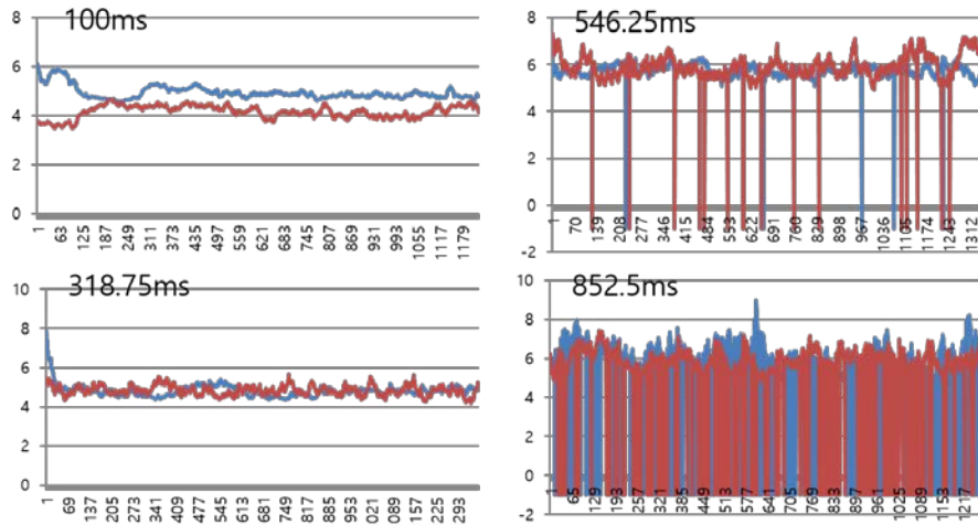
Fig. 10. Measured signal
