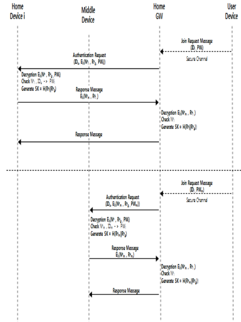
Fig. 4. User Device Access Protocol
