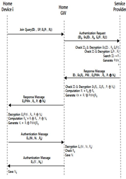
Fig. 2. Device Addition Protocol
