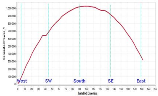
Fig. 20. Simulation result of the installed direction
