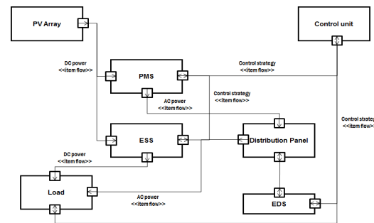
Fig. 12. ibd model for BIPV power generation system
