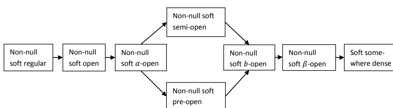
FIGURE 1. The relationships between soft somewhere dense set and some generalized soft open sets
