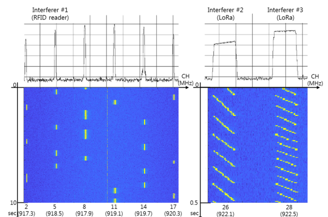
Fig. 8. Spectrogram of the interference signals (RFID and LoRa) on each channel.
