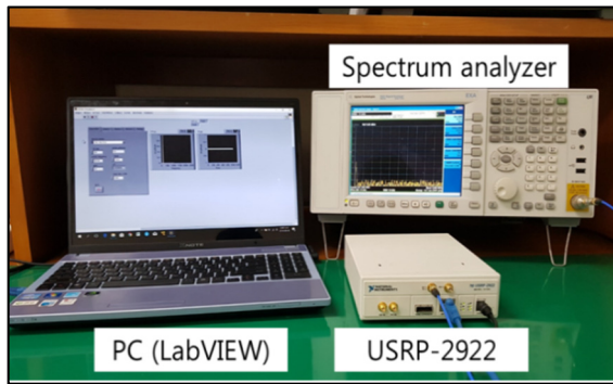
Fig. 6. Configuration of the verification experiment for the proposed emulator.
