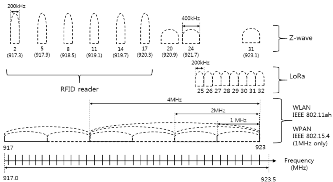
Fig. 1. Channel allocation in the Korean RFID/USN frequency band (917–923.5 MHz).
