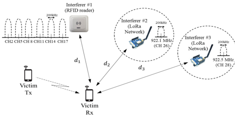
Fig. 2. Interference scenario of the Korean RFID/USN band.
