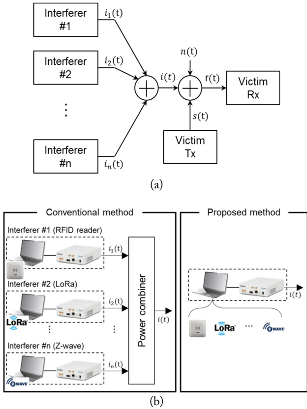
Fig. 3. Emulation for the interference environment: (a) the interference signal generator using multiple signal generators and (b) the interference signal emulator using only one signal generator with a heterogeneous signal generation function.
