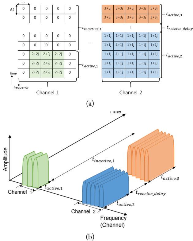
Fig. 4. Concept of the heterogeneous interference emulator: (a) the matrix form and (b) the signal generation for the matrix form.
