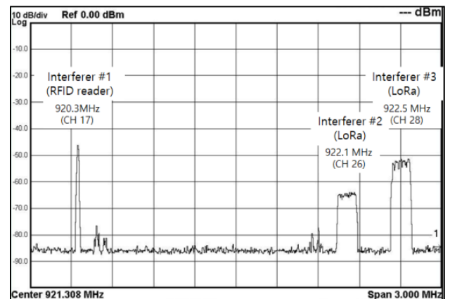
Fig. 7. PSD of the multiple interference signals (Max hold).
