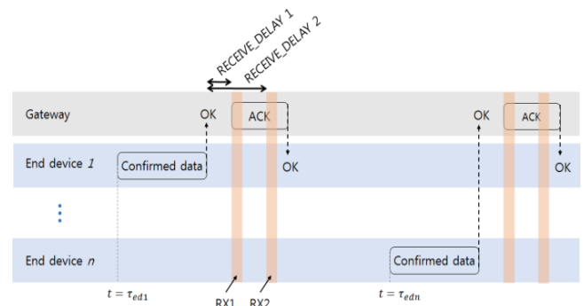
Fig. 5. Example of a LoRa uplink timing diagram for a confirmed data message in a class A feature.
