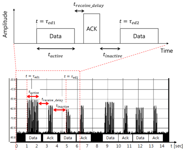
Fig. 9. Interference signal of the LoRa network on channel 28 (time domain).
