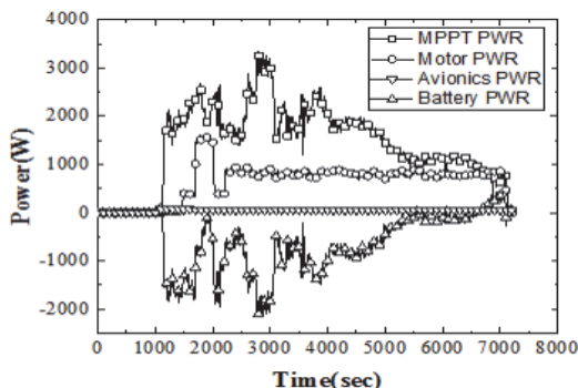
Fig. 12 Power balance.
