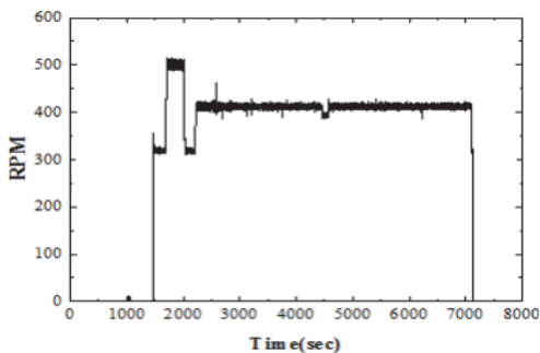
Fig. 11 RPM command.
