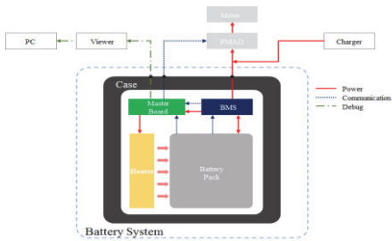
Fig. 3 Battery system.
