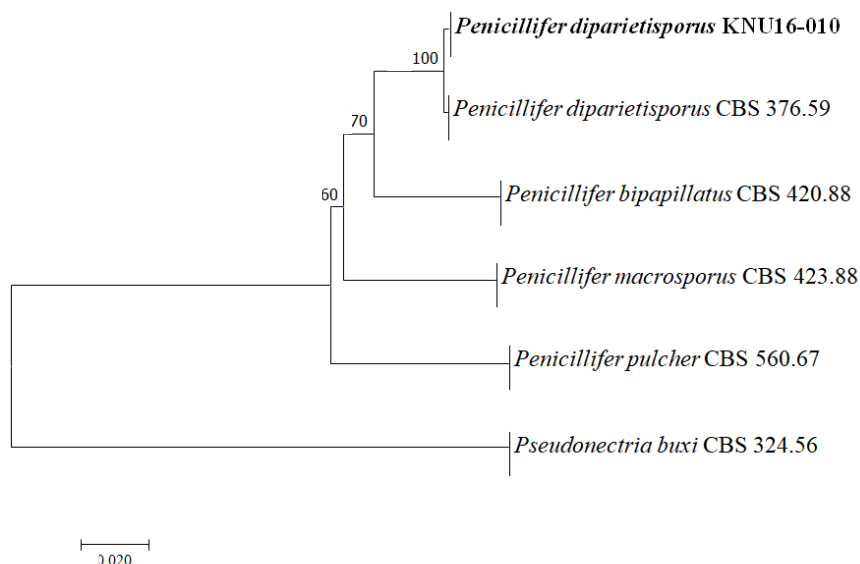
Fig. 3. Neighbor-joining phylogenetic tree based on the combined internal transcribed spacer sequences and translation elongation factor 1- \alpha . Pseudonectria buxi CBS 324.56 was used as an outgroup. The strain isolated in this study is indicated in bold, and the bootstrap values are based on 1,000 replications. Bar, 0.02 substitutions per nucleotide position.
