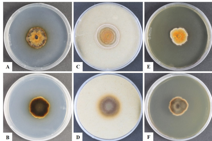
Fig. 1. Cultural characteristics of KNU16-010. A, B, Front and reverse sides of the colony on potato dextrose agar; C, D, Front and reverse sides of the oatmeal agar; E, F, Front and reverse sides of the malt extract agar.
