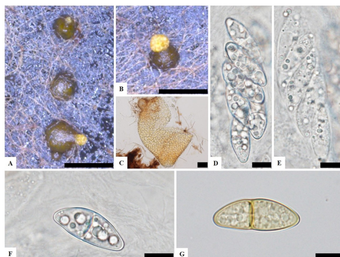
Fig. 2. Morphological characteristics of KNU16-010. A, B, Mature perithecia on potato dextrose agar; C, Perithecium; D, E, Asci; F, G, Ascospores (scale bars: A, B = 500 \mu m, C = 50 \mu m, D-G = 10 \mu m).
