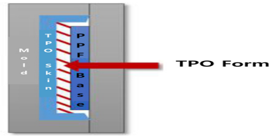
Fig. 2. Ejecting method of high-sensibility door trim
