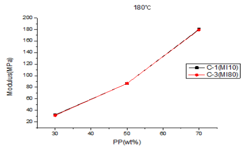
Fig. 16. Modulus of TPE in Como-PP at 180°C
