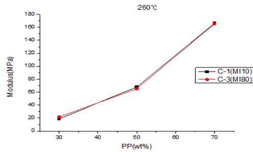
Fig. 18. Modulus of TPE in Como-PP at 260°C
