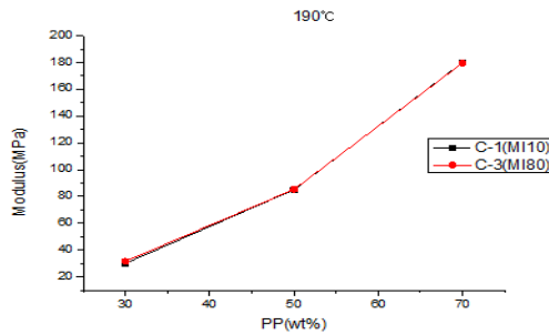
Fig. 17. Modulus of TPE in Como-PP at 190°C
