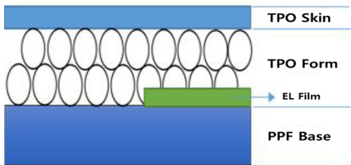
Fig. 1. Structure of high-sensibility door trim
