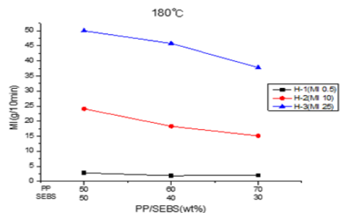
Fig. 7. MI of Homo-PP% at 180°C
