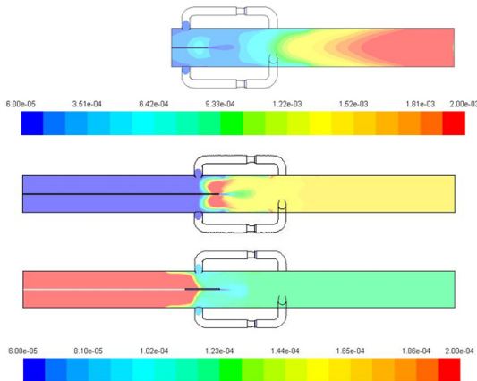
Fig. 7. Contours of NOx concentration distribution at the section of x=0mm
