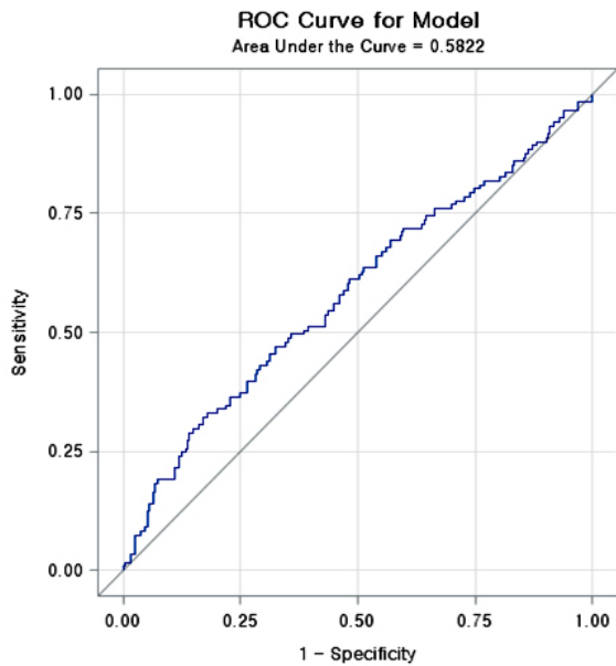
Fig. 4. ROC curve for the NQ model
