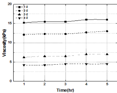
(b) RDX 1 & RDX 2 mixing ratio = 30.0 : 14.0
