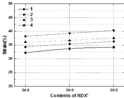
Fig. 4 Strain of propellants with different particle size of RDX.
