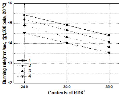
Fig. 5 Burning rate of propellants with different particle size of RDX. (@1,500 psia, 20 °C).
