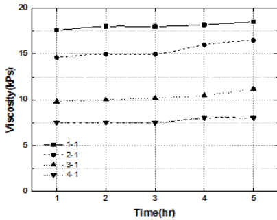
(a) RDX 1 & RDX 2 mixing ratio = 24.0 : 20.0
