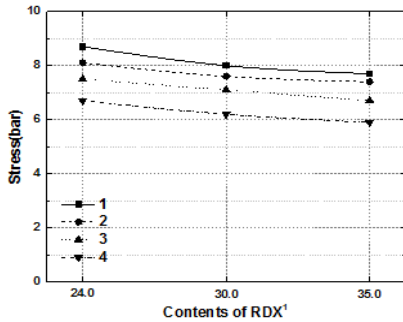
Fig. 3 Stress of propellants with different particle size of RDX.
