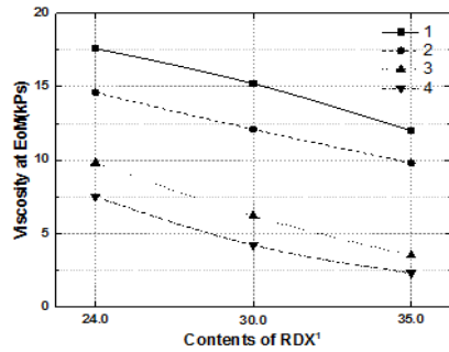
Fig. 2 Viscosity of propellants with different particle size of RDX.
