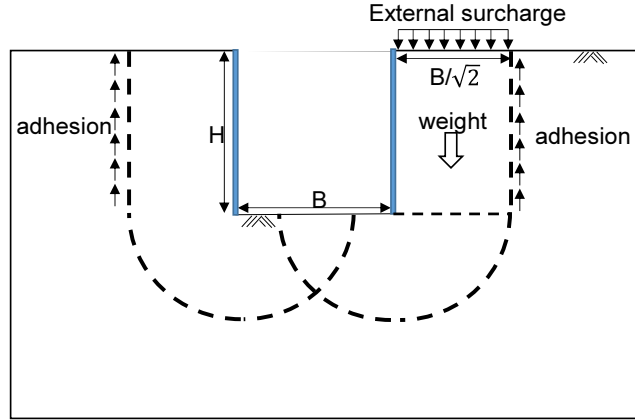
Fig. 3. Conceptual diagram of driving force and resisting force (Terzaghi and Peck, 1948)
