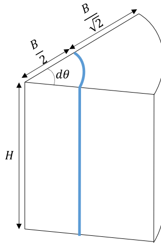
Fig. 4. Conceptual diagram for considering 3D geometry
