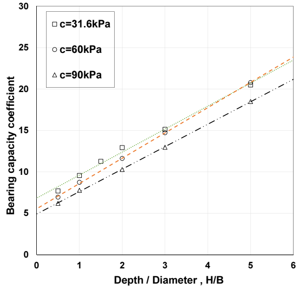
Fig. 8. Bearing capacity coefficient variation with increasing depth - effect of cohesion (B = 10 m)
