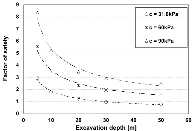
Fig. 6. Factor of safety variation with increasing depth - effect of cohesion (B = 10 m)
