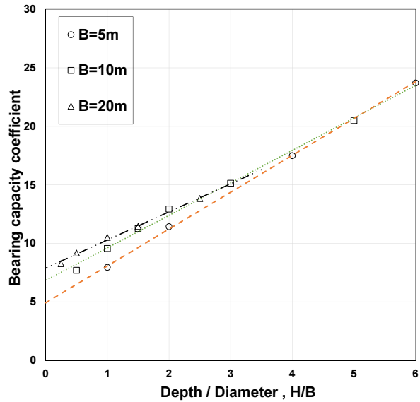
Fig. 9. Bearing capacity coefficient variation with increasing depth - effect of diameter (c = 31.6 kPa)
