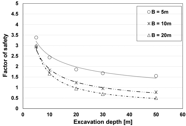
Fig. 7. Factor of safety variation with increasing depth - effect of diameter ( c = 31.6 kPa)
