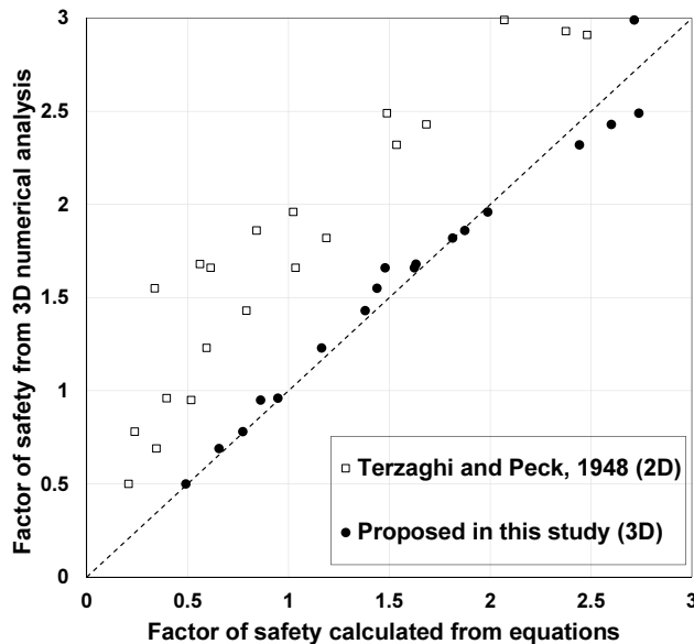
Fig. 10. Comparison of factor of safety from numerical analysis and equations
