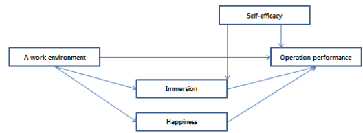
Fig. 3. Research model
