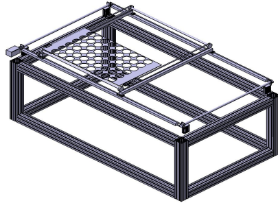
Fig. 10. Fixture unit
