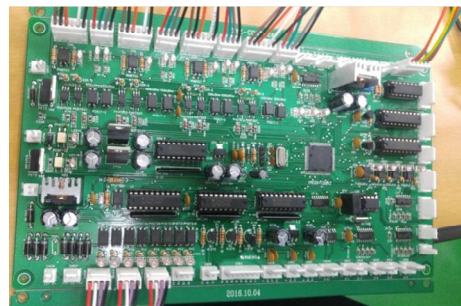
Fig. 14. Control board
