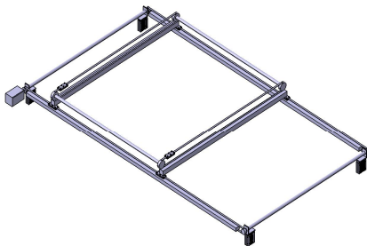
Fig. 9. Conveying unit
