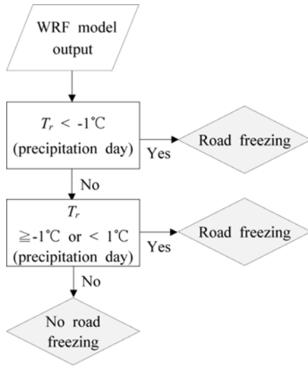
Fig. 3. Flowchart for road freezing prediction algorithm developed by Imacho et al (2002).
