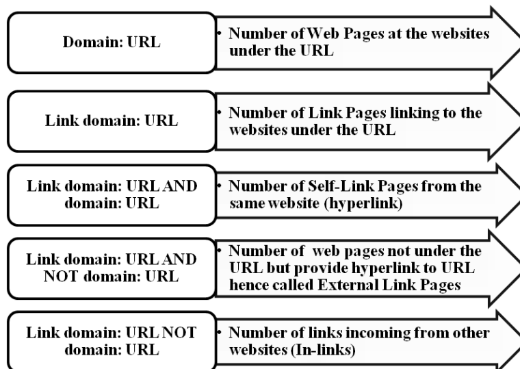
Fig. 2. Webometric query syntax supported by Google with results
