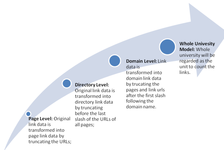
Fig. 3. Four parts of the Alternative Document Model (ADM)
