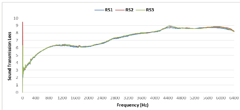
Fig. 7. Transmission loss of the rice-straw mat of thickness 5 mm and apparent specific density 0.12 \text{ g/cm}^3 .
