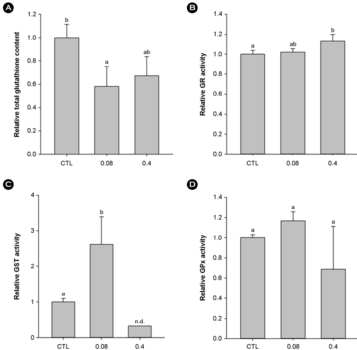
Fig. 2. Modulation of oxidative stress markers in Diaphanosoma celebensis exposed to HgCl 2 (0.08 and 0.4 mg/l) for 24 h. (A) total glutathione content, (B) GR activity, (C) GST activity, and (D) GPx activity. Data are shown as means \pm S.D. of three replicates. Significant differences between different concentrations were determined by one-way analysis of variance (ANOVA), followed by Turkey's test, and are indicated using lowercase letter. n.d. (not detected).
