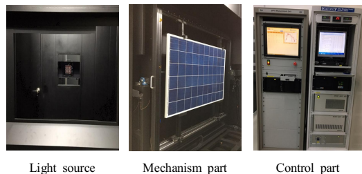
Fig. 1. Composition of BIPV Measurement system
