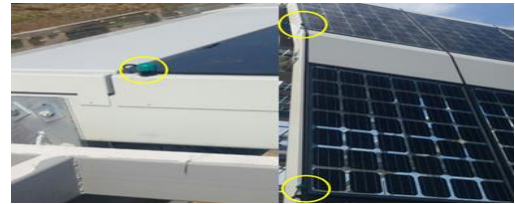
Irradiation sensor for installation angle and azimuth
