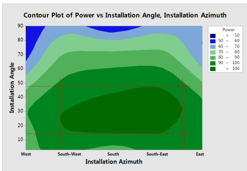
Fig. 18. Contour plot analysis for power generation of design elements(c-Si, installation azimuth and angles)
