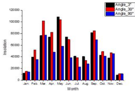
Fig. 13. Comparison monthly cumulative insolation for installation angles(3°, 30°, 90°)
