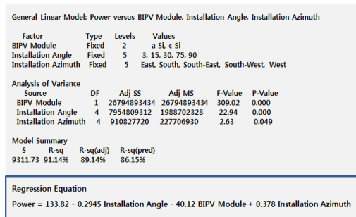
Fig. 17. Regression analysis for power generation of design elements(module, installation azimuth and angles)
