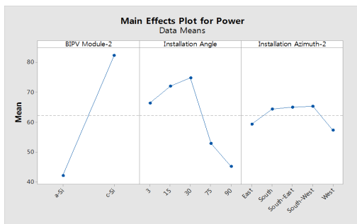
Fig. 15. Main effect plot analysis for design elements (BIPV module, installation azimuth and angles)
