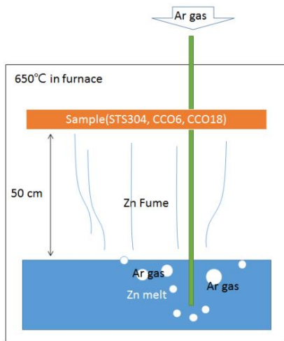
Fig. 2. Zn fume corrosion test device
