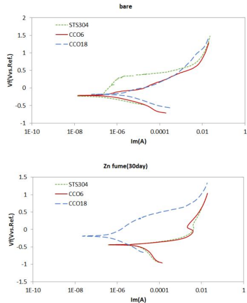
Fig. 5. Potentiodynamic polarization graph
