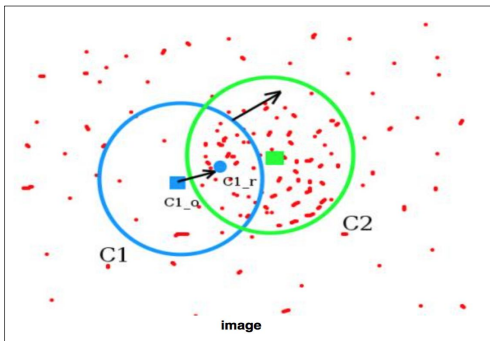
Fig. 8. Mean-Shift Method
