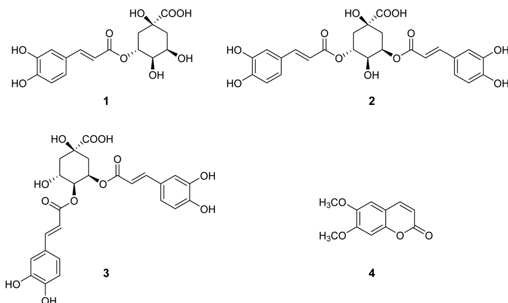
Fig. 1. Structures of four standards, chlorogenic acid (1), 3,5-dicaffeoylquinic acid (2), 4,5-dicaffeoylquinic acid (3) and scoparone (4), from A. capillaris .
