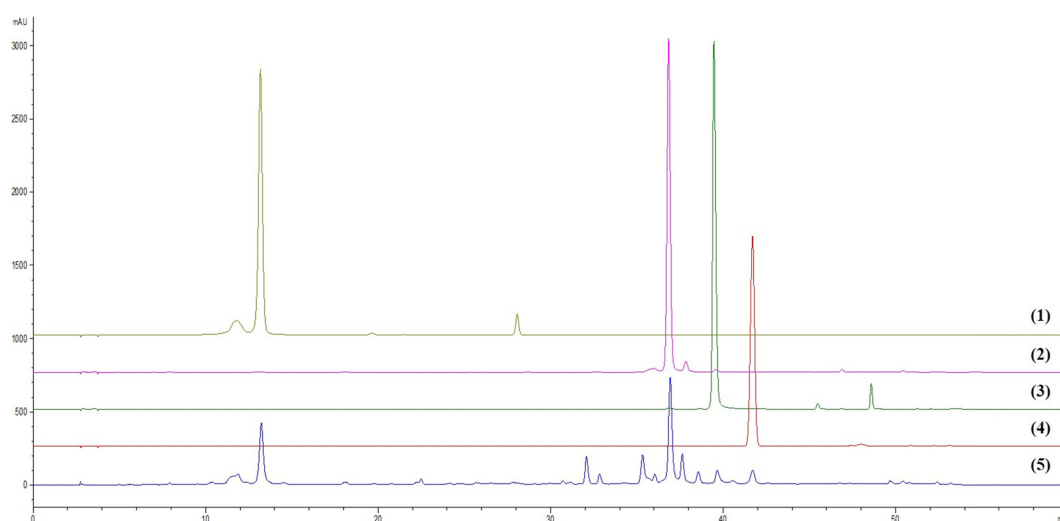
Fig. 2. HPLC chromatogram of four standards, chlorogenic acid (1), 3,5-dicaffeoylquinic acid (2), 4,5-dicaffeoylquinic acid (3), scoparone (4), and the 70% ethanolic extract of A. capillaris (5).
