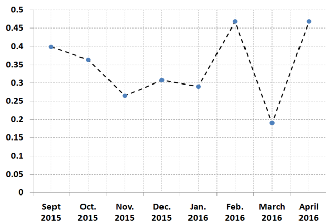
Fig. 4. Monthly average PM_{2.5}/PM_{10} ratios.
