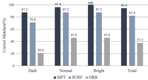
〈Figure 11〉 Evaluation Results for Illumination Invariance
