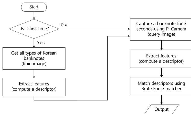
<Figure 2> Banknote Recognition Flowchart
