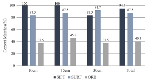
〈Figure 13〉 Evaluation Results for Scale Invariance
