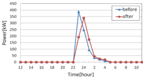
Fig. 7. Charging power of PEVs applying system constraints
