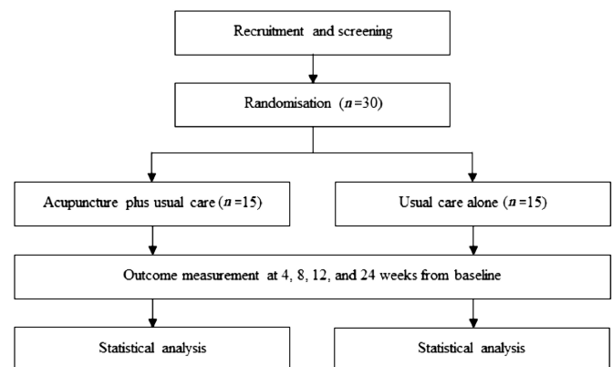
Fig. 1. Trial flowchart.
