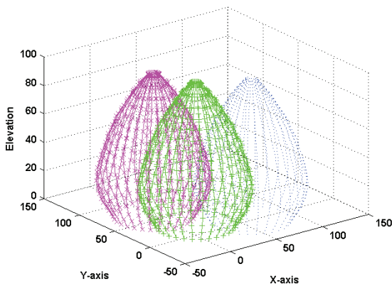
Fig. 5. The surface plot of the three-dimensional VL positioning channels constructed by three VL transmitters in a real VL positioning environment similar to Fig. 1
