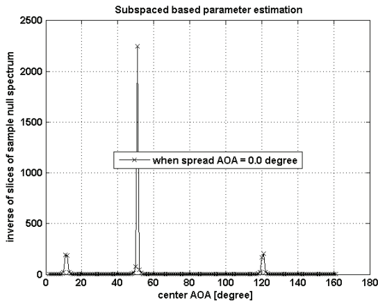
Fig. 8. The inverse plot of the two-dimensional slices of the three-dimensional sample null spectrum of Fig. 6 under the condition that the AOA is assumed the point form like Fig. 2(a)
