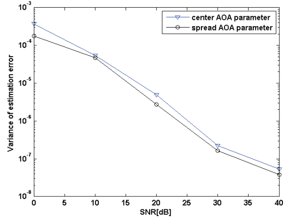
Fig. 9. Variances of the center and spread AOA estimation errors of the subspace-based AOA estimation technique
