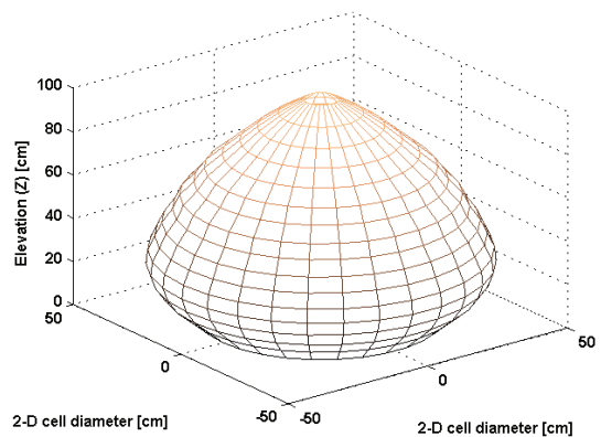
Fig. 4. The surface plot of the three-dimensional VL channel by one VL signal source obtained in a real VL positioning test
