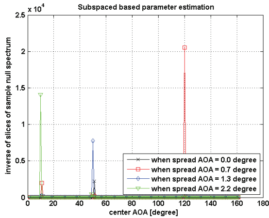
Fig. 7. The inverse plot of the two-dimensional slices of the three-dimensional sample null spectrum of Fig. 6 under the condition that the spread AOA parameter is given
