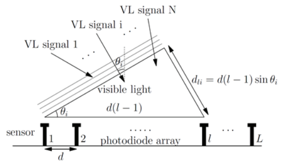
Fig. 3. The reception process of the VL signals acquired at the receiver of the photodiode array of uniform linear array sensor
