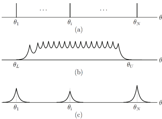
Fig. 2. Three forms of the AOA parameter observed at the receiver under the real VL positioning channel (a) a point angle form (b) a random and nonparametric distributed angle form (c) a random and parametric distributed angle form
