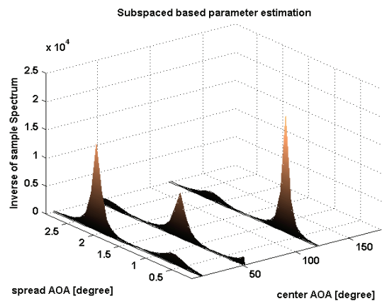
Fig. 6. The inverse plot of the sample null spectrum obtained by the subspace-based AOA estimation technique for short range VL positioning as written in Eq. (13)
