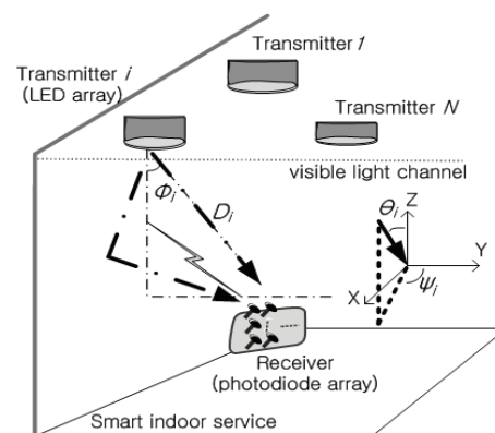
Fig. 1. The channel environment of the VL positioning methodology based on the AOA parameter estimation for the smart indoor service
